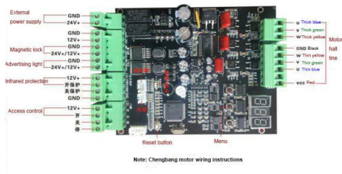
Control Board
