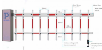
Size Diagram of Hot-Sale Fence Gate
